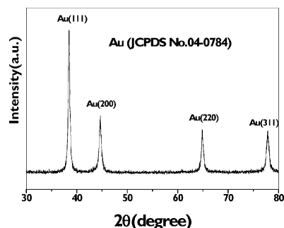
Fig. 1 X-Ray diffraction pattern of GNPs–GNSs nanocomposite.
