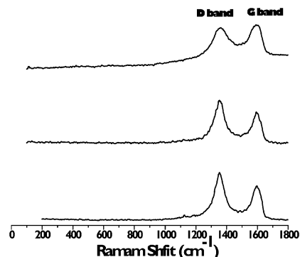
Fig. 3 Raman spectra of GO (top), GNSs (middle) and GNPs–GNSs (bottom).
